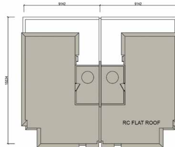
Roof Plan
