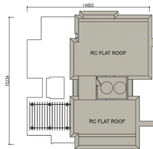
Roof Plan
